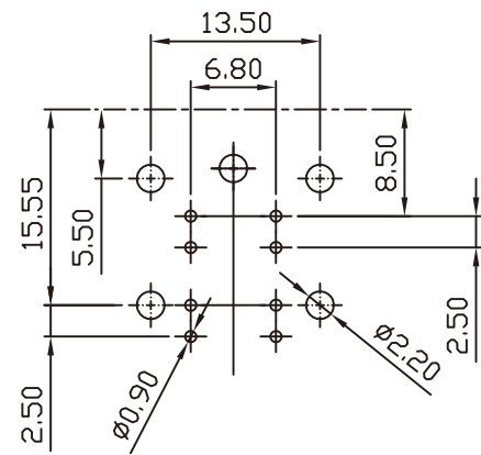
RECOMMAND PC BOARD HOLE LAYOUT
