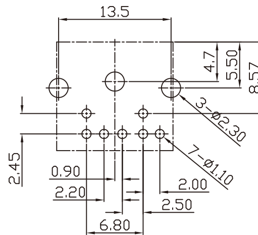
RECOMMAND PC BOARD HOLE LAYOUT
