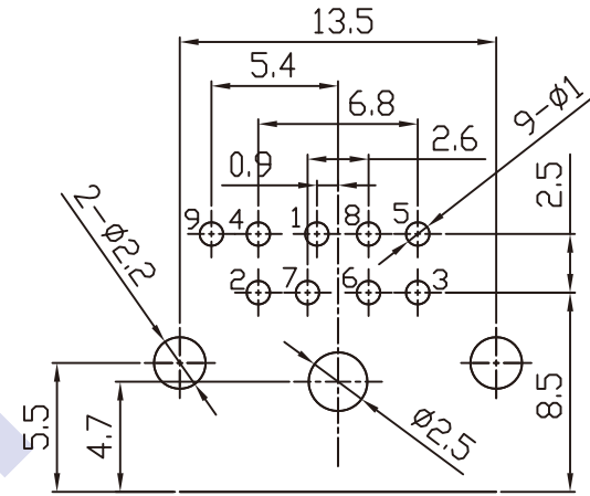
RECOMMEND PC BOARD HOLE LAYOUT
